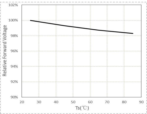
Fig 6. Soldering Temperature vs. Relative Forward Voltage (IF=60mA)
