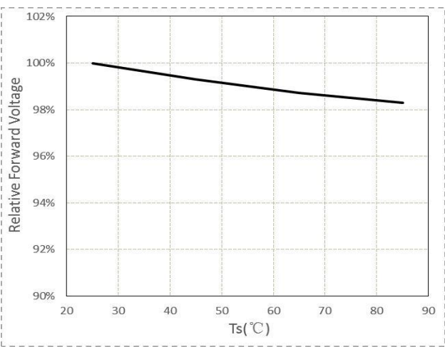
Fig 6. Soldering Temperature vs. Relative Forward Voltage (IF=150mA)
