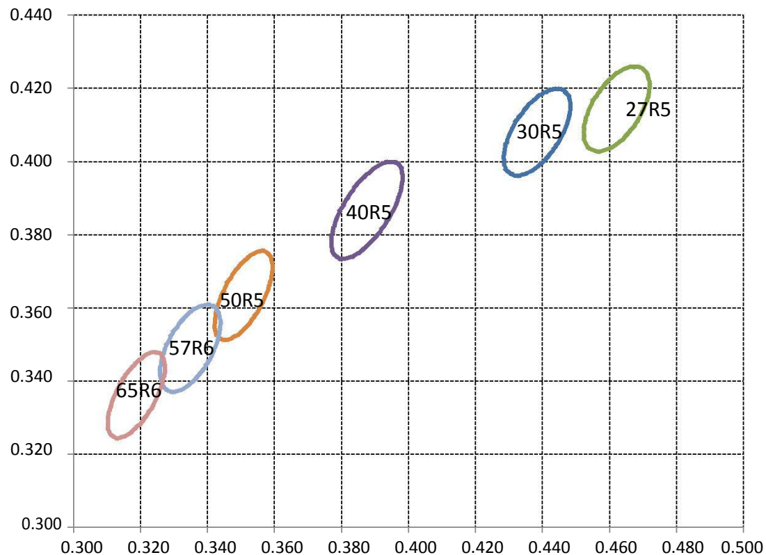
Fig 9, CIE Chromaticity Diagram (CIE 色区图), IF = 30mA, Ta = 25°C
